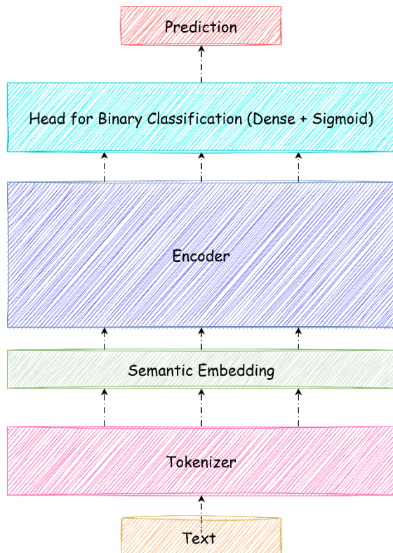
Figure 1 : Model Architecture
